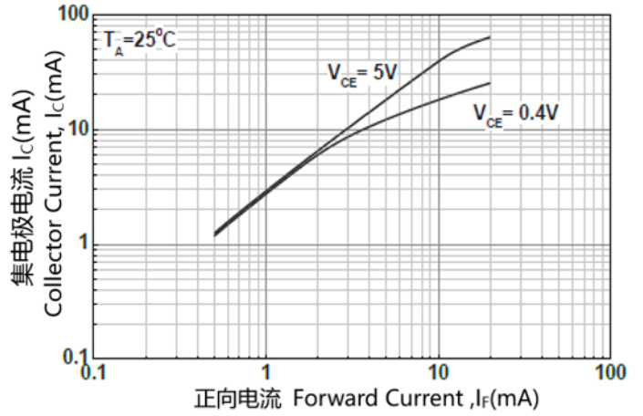
Figure2.Collector Current vs Forward Current
