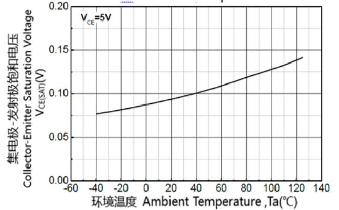
Figure 10. Collector-Emitter Saturation Voltage vs Ambient Temperature
