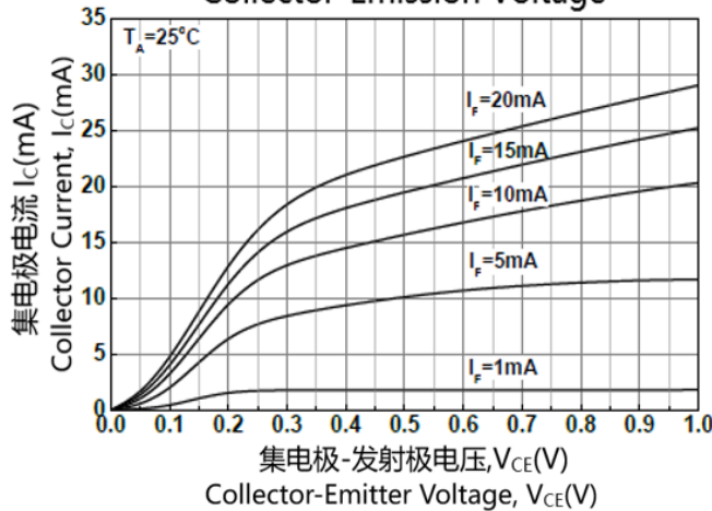
Figure5. Collector Current vs Collector-Emission Voltage
