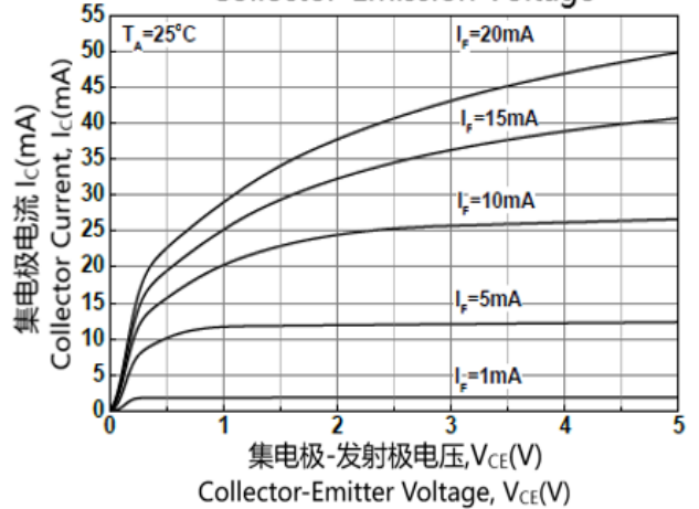
Figure4. Collector Current vs Collector-Emission Voltage
