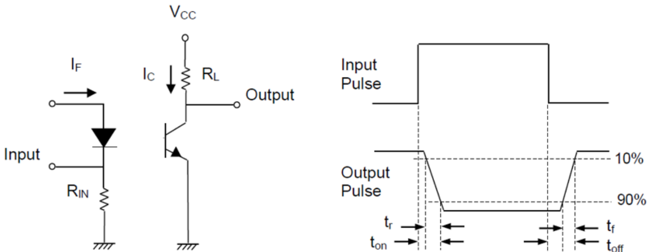
Figure 11. Switching Time Test Circuit & Waveforms
