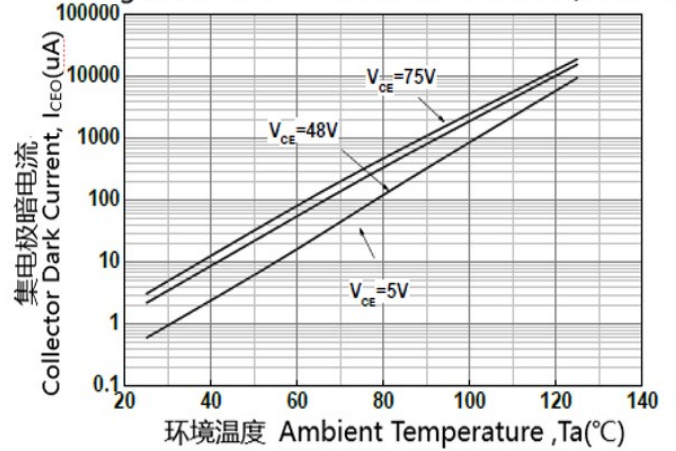
Figure 8. Dark Current vs Ambient Temperature
