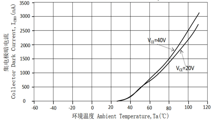
Collector Dark Current vs Ambient Temperature
