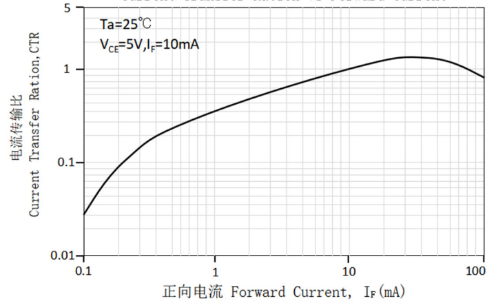
Current Transfer Ratio vs Forward Current
