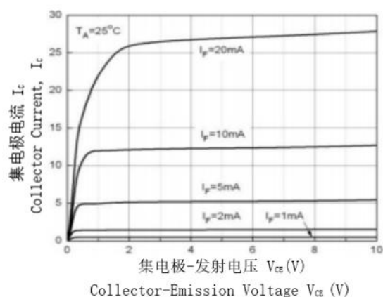
Fig.6 Collector current vs Collector-Emission Voltage
