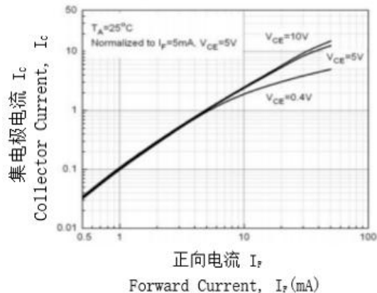
Fig.2 Collector Current vs Forward Current
