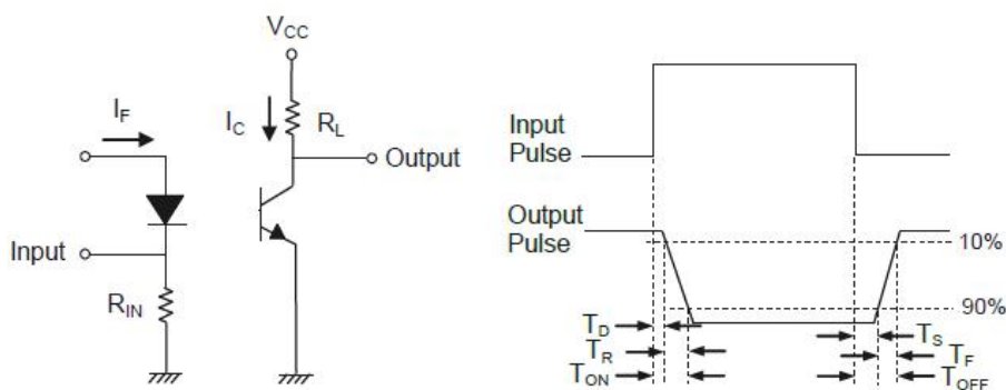
Fig.11 Switching Time Test Circuit &amp; Waveforms
