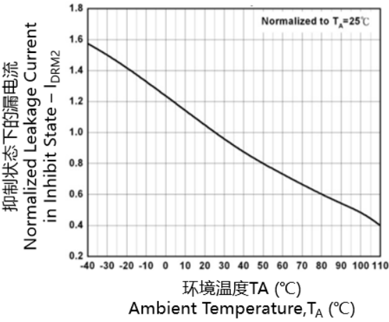
图8. 抑制状态下的漏电流 vs 环境温度的关系 Figure 8. Leakage Current in Inhibit State vs Ambient Temperature
